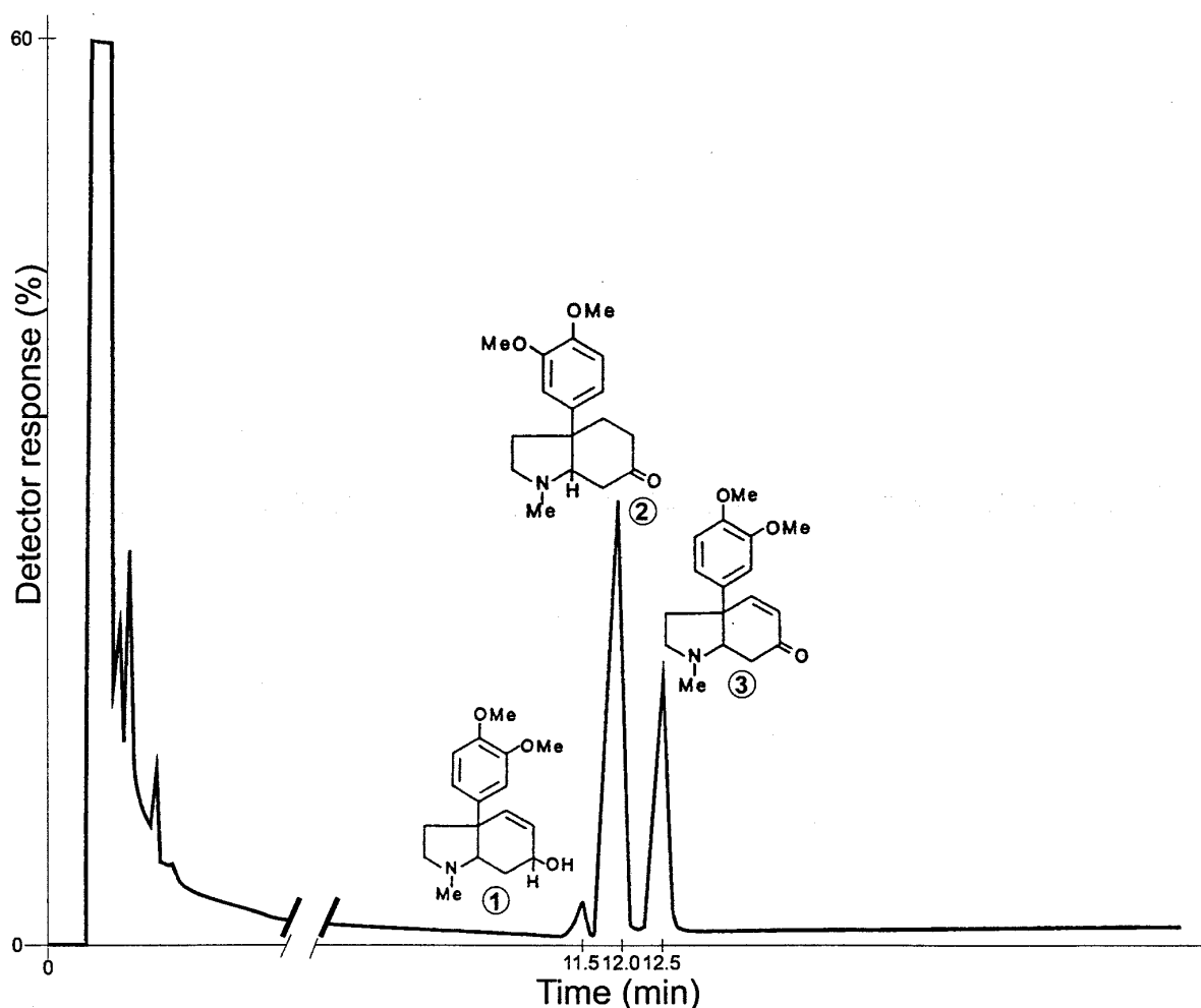
Fig. 1. Chromatogram of Scaletium tortuosum showing three mesembrine alkaloid peaks; 1. 4'- O -demethylmesembrenol, 2. mesembrine and 3. mesembrenone.
