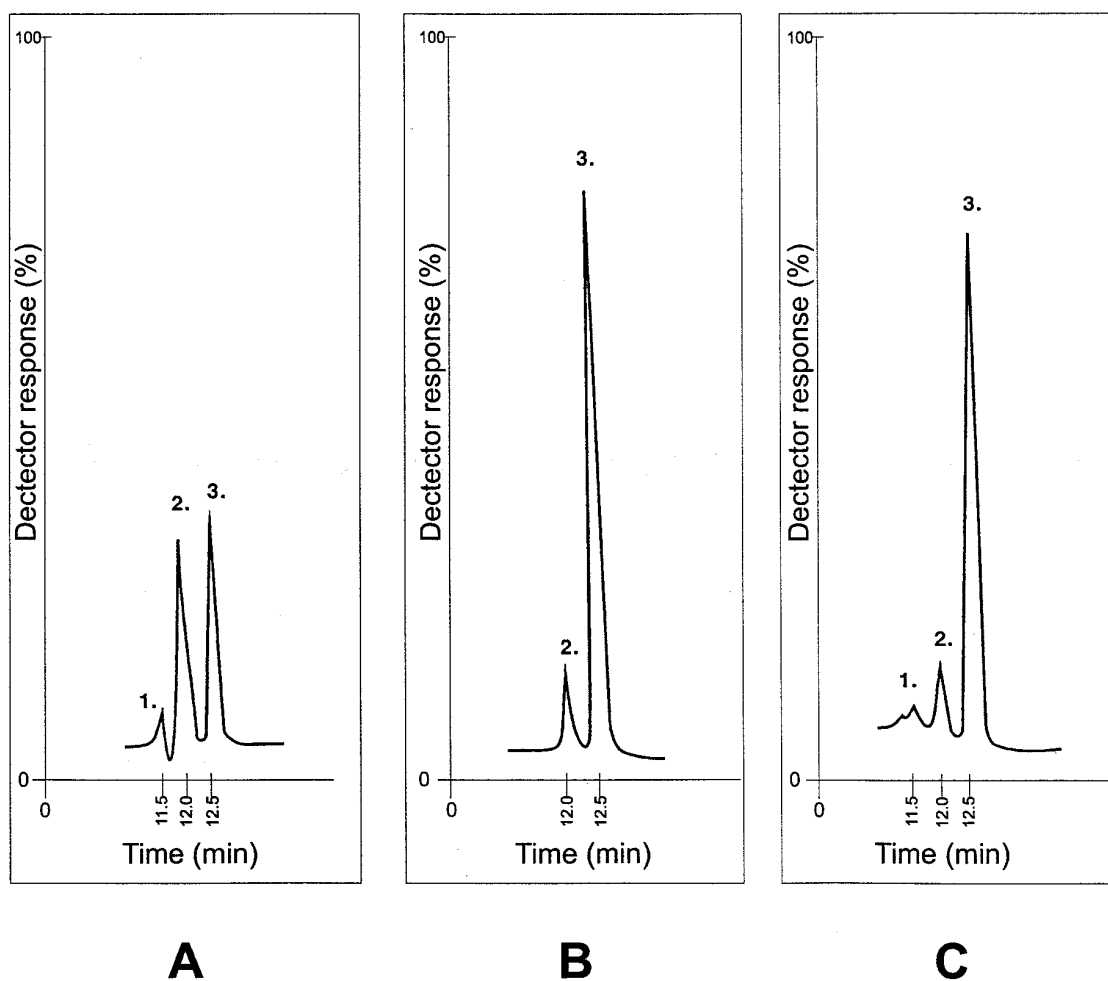
Fig. 2. Chromatographic profiles of Sceletium tortuosum extracts showing the different levels of 1. 4'- O -demethylmesembrenol, 2. mesembrine and 3. mesembrenone for: (A) uncrushed plant material dried at 80°C, (B) crushed and fermented plant material and (C) crushed plant material dried at 80°C.
